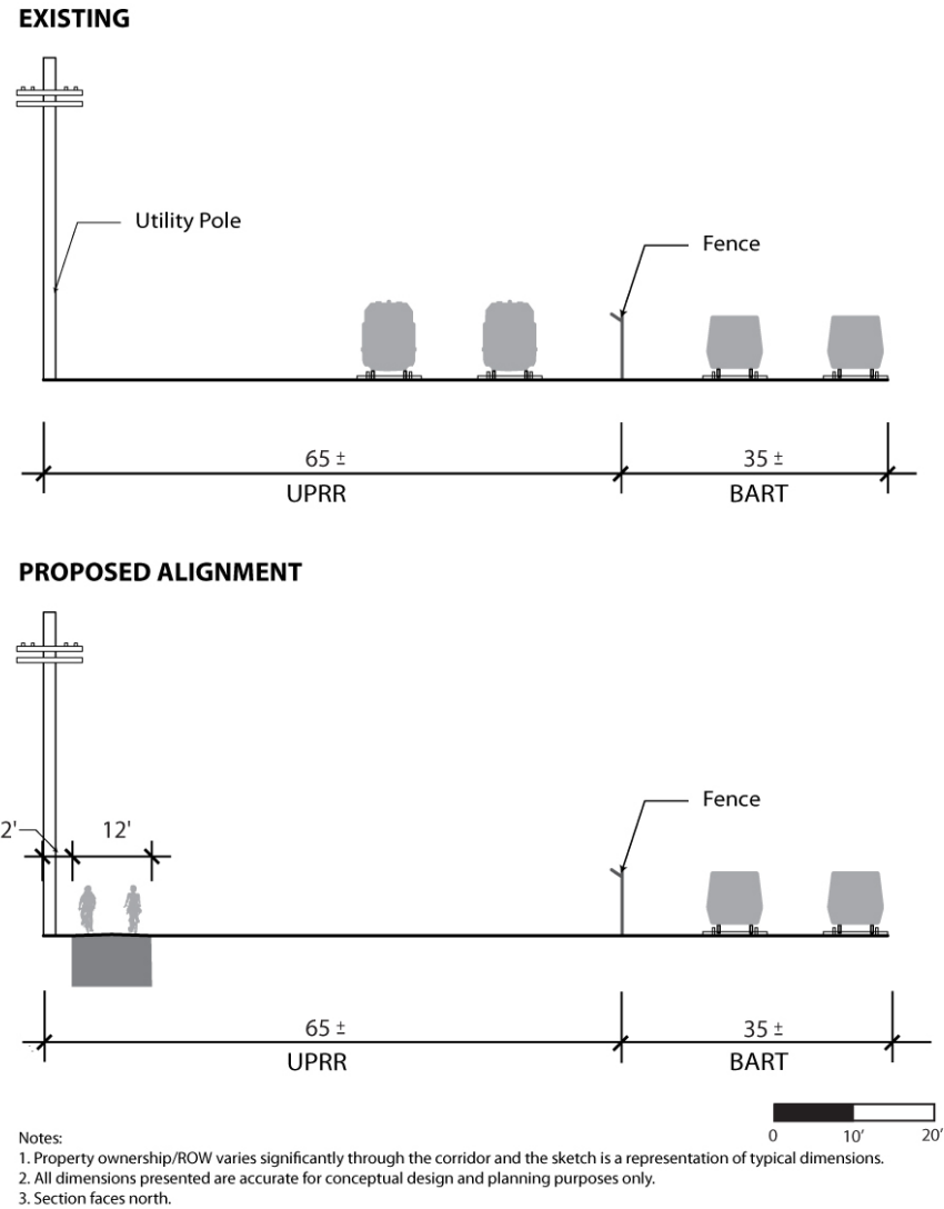
Figure 4-20: Proposed Segment 3.5 Alignment
