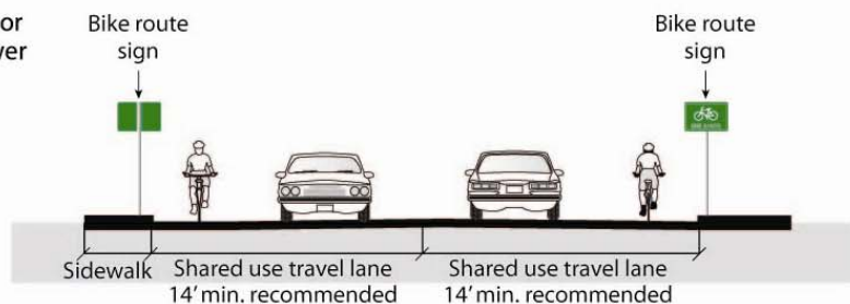
Figure 3-1: Bike Route Classifications
