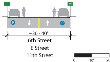
Figure 4-28: Proposed Segment 5.1 Alignment
