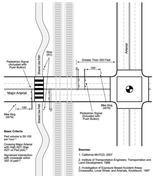
Roadway crossing type 2 (new signal)
