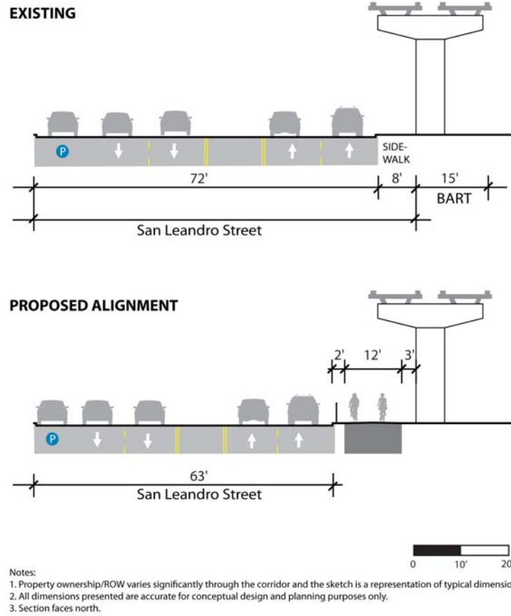
Figure 4-9: Proposed Segment 1.5 Alignment
