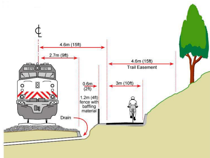
Figure 3-4: Rail-with-Trail Constraints
